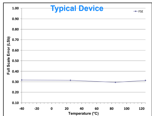
FIGURE 2-30: Full-Scale Error (FSE) vs. Temperature. V_{DD} = 3.0\text{V} , V_{REF} = 1.65\text{V} .
