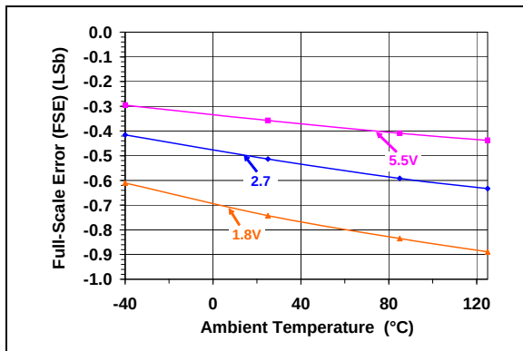
FIGURE 2-27: 10 kΩ : Full Scale Error (FSE) vs. Temperature ( V_{DD} = 5.5\text{V} , 2.7V, 1.8V).
