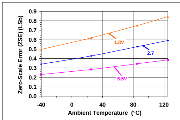
FIGURE 2-28: 10 kΩ : Zero Scale Error (ZSE) vs. Temperature ( V_{DD} = 5.5\text{V} , 2.7V, 1.8V).
