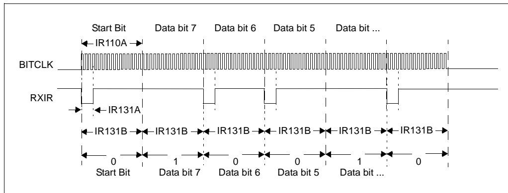
FIGURE 4-9: RXIR WAVEFORMS
