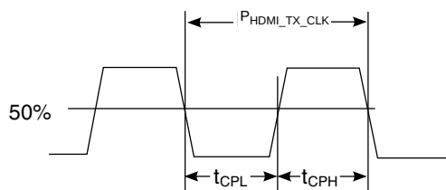
Figure 54. TMDS Clock Signal Definitions
