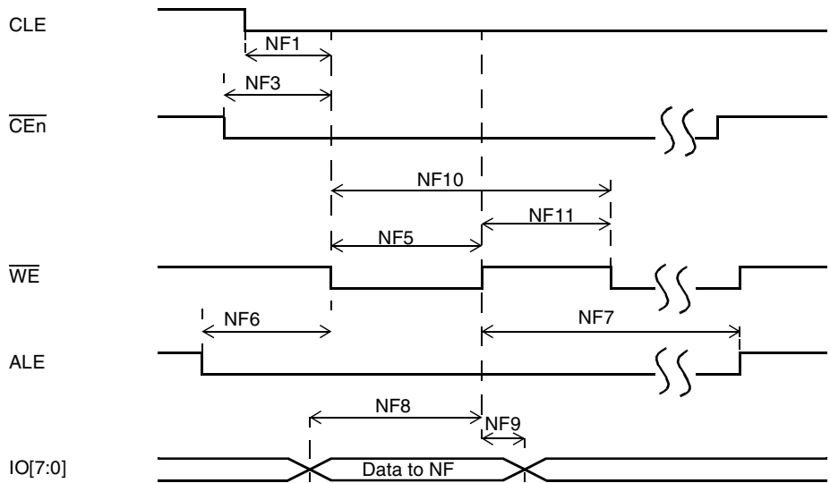
Figure 22. Write Data Latch Cycle Timing Diagram
