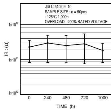
Fig.21 Insulation resistance
