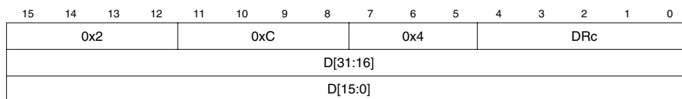
Figure A-5. Write Debug Module Register Command (WDMREG)
