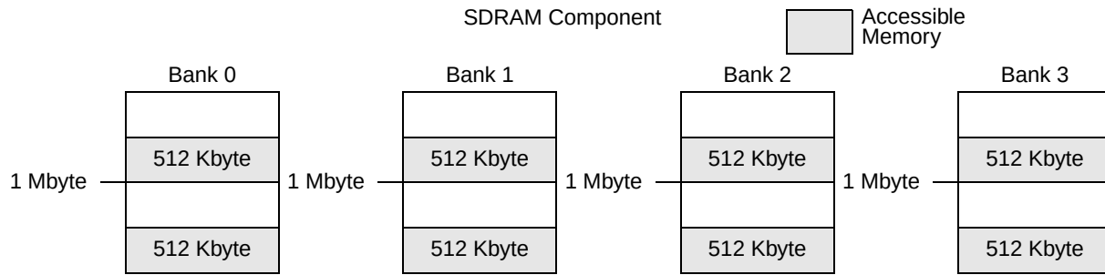
Figure 15-12. SDRAM Configuration
