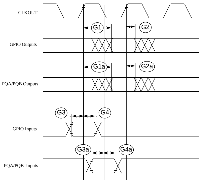
Figure 33-8. GPIO Timing
