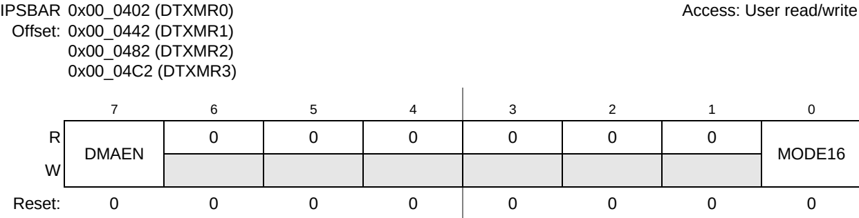
Figure 21-3. DTXMRn Registers
