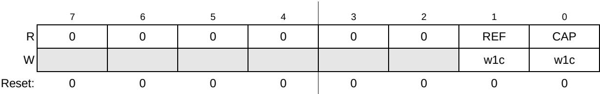
Figure 21-4. DTERn Registers
