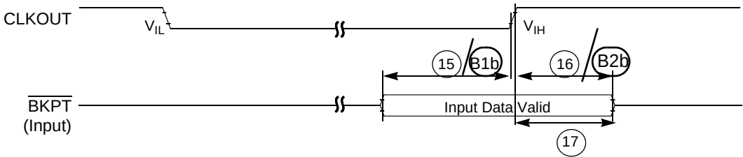
Figure 33-20. \overline{\text{BKPT}} Timing
