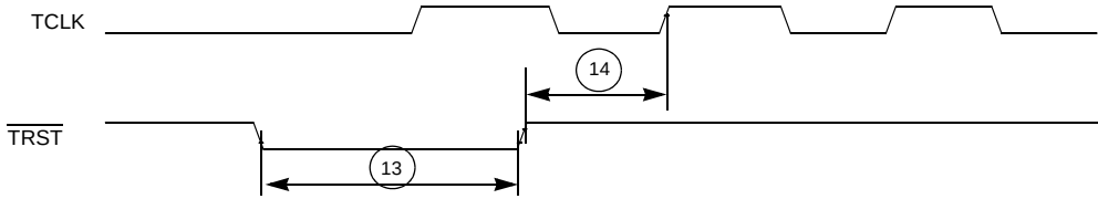
Figure 33-19. \overline{\text{TRST}} Timing
