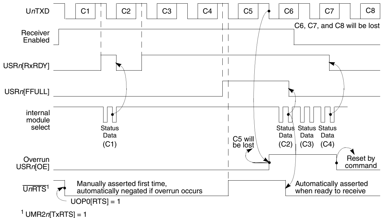
Figure 24-20. Receiver Timing
