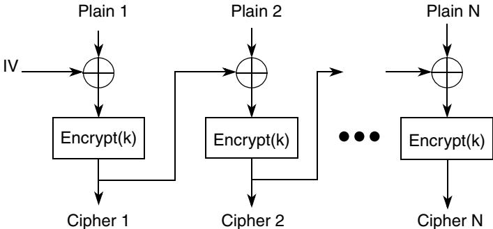
Figure 28-5. CBC Encryption
