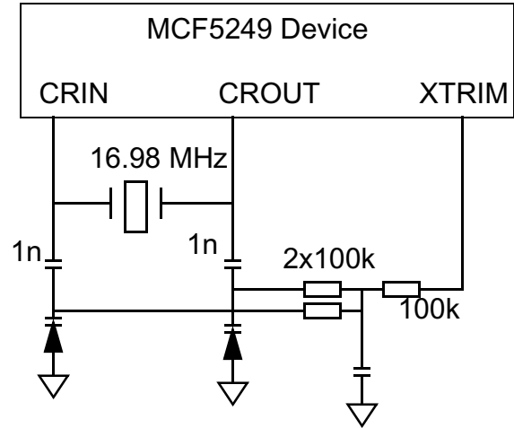
Figure 17-12 XTRIM External Circuit
