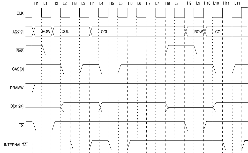
Figure 10-13. Word Read Transfer Followed by a Page Miss Byte Read Transfer in Fast Page Mode with 8-Bit EDO DRAM
