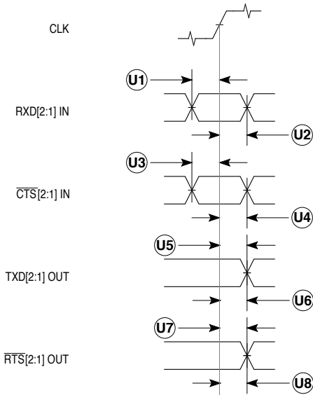
UART Timing
