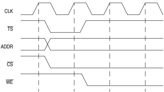
Figure 8-11. Chip Select and Write-Enable Assertion with ASET = 0 Timing
