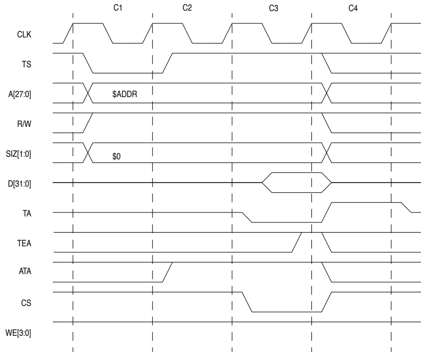
Figure 8-8. Alternate Master Longword Read Transfer from a 32-Bit Port (No Wait State, No Address Setup, No Address Hold)
