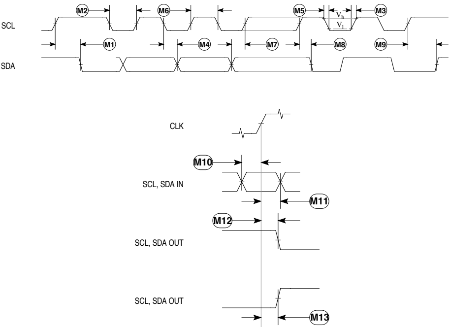
M-Bus Timing
