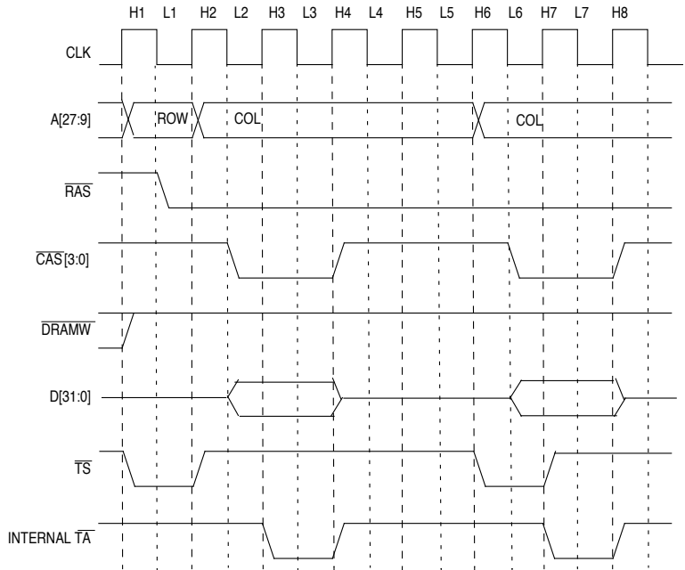
Figure 10-8. Longword Read Transfer Followed by a Page Hit Longword Read Transfer in Fast Page Mode with 32-Bit DRAM
