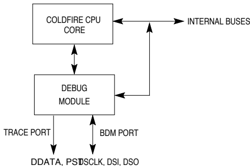
Figure 14-1. Processor/Debug Module Interface
