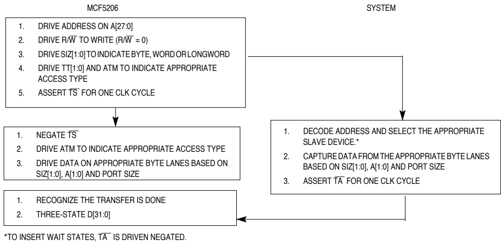
Figure 6-6. Byte-, Word-, and Longword-Write Transfer Flowchart
