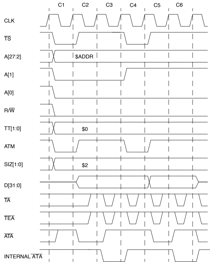
Figure 6-27. Burst-Inhibited Longword-Write Transfer to 16-Bit Port Using Asynchronous Termination (One Wait State)
