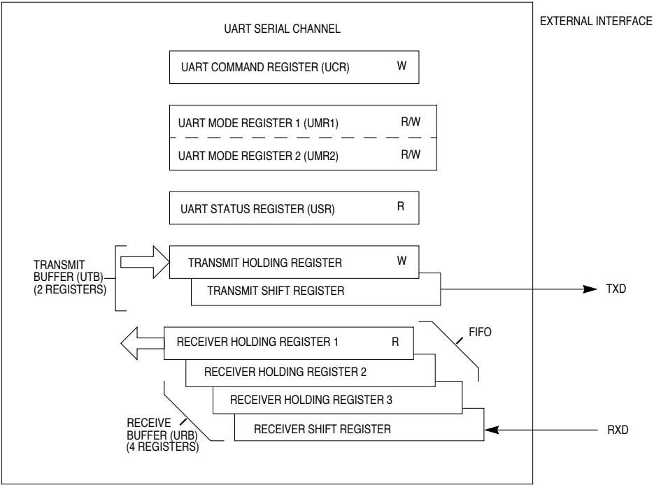
Figure 11-4. Transmitter and Receiver Functional Diagram
