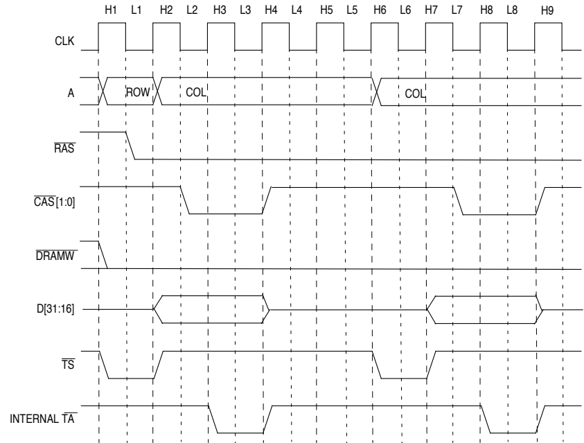
Figure 10-9. Word Write Transfer Followed by a Page-Hit Word Write Transfer in Fast Page Mode with 16-bit DRAM
