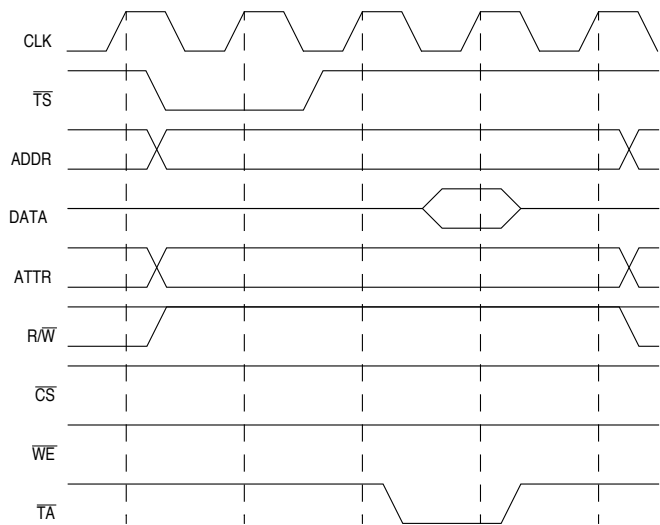
Figure 8-20. Default Memory Address Hold Timing with RDAH = 1
