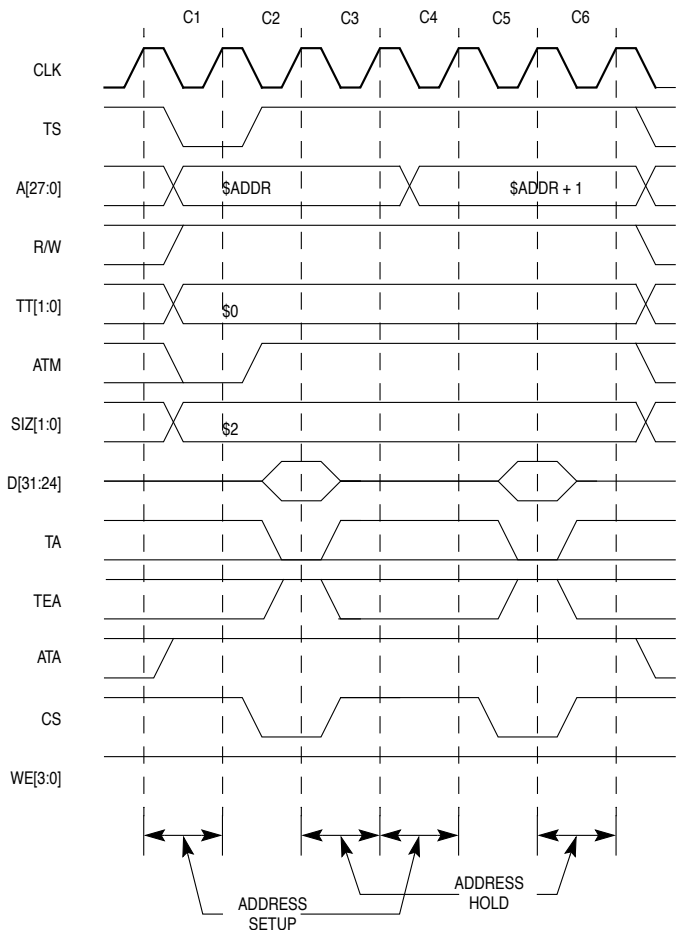
Figure 8-7. Word Burst Read Transfer from an 8-Bit Port (No Wait States, Address Setup, Address Hold)
