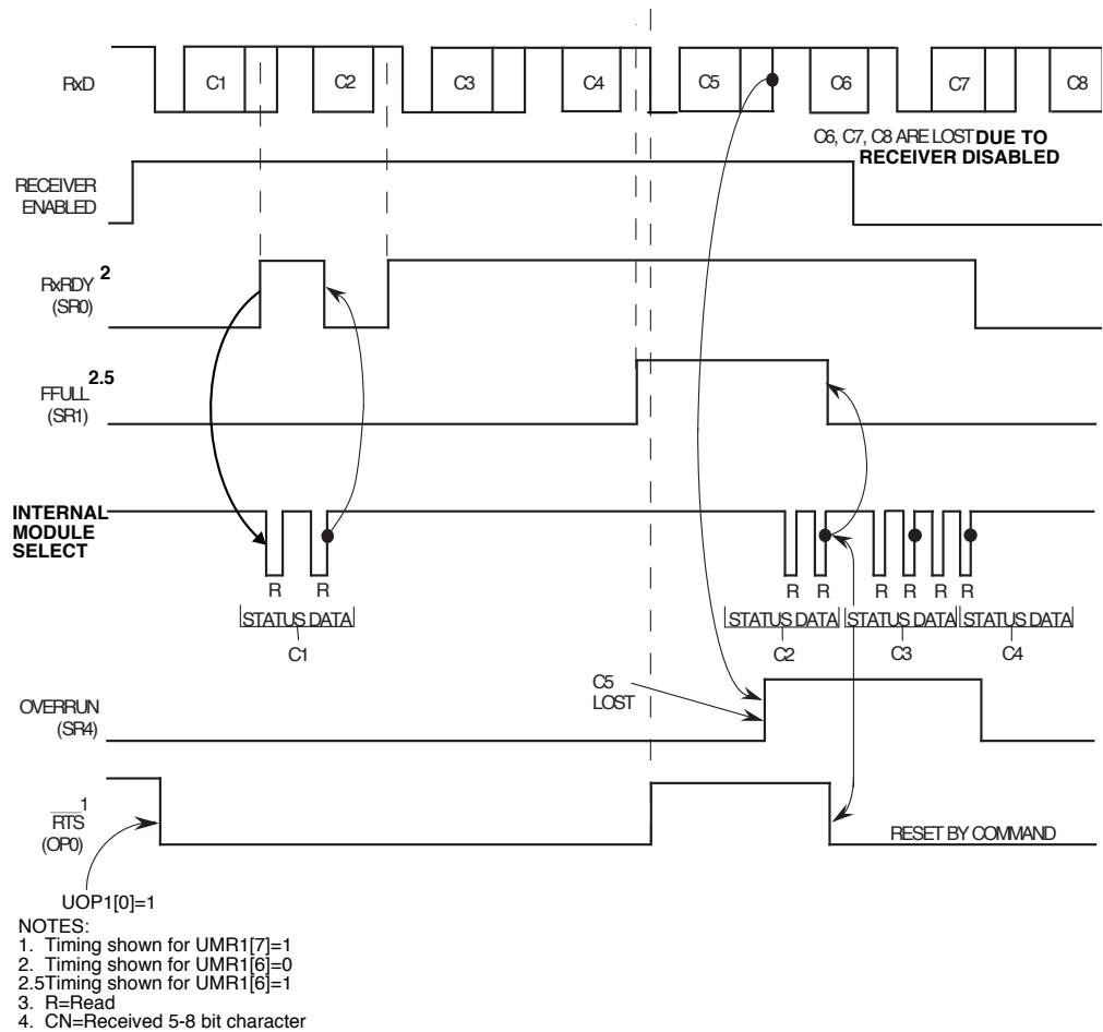
Figure 11-6. Receiver Timing Diagram
