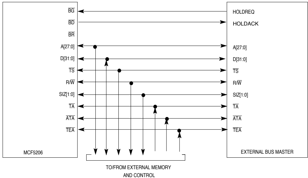
Figure 6-33. MCF5206 Two-Wire Mode Bus Arbitration Interface
