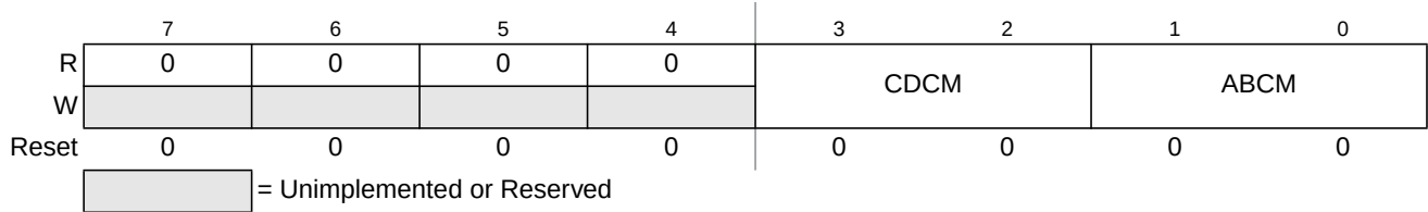
Figure 22-6. Debug Control Register2 (DBGCR2)
