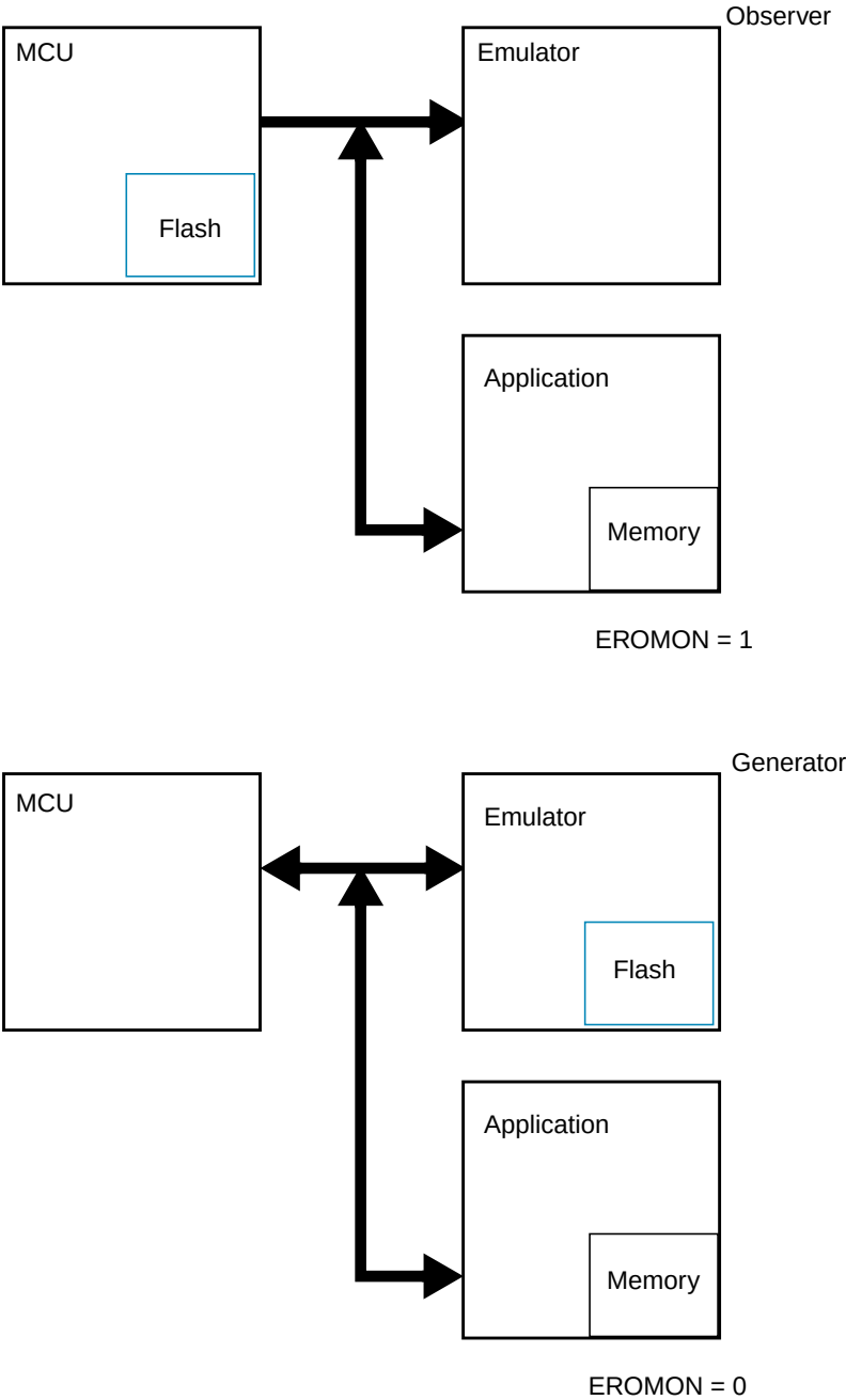
Figure 25-30. ROMON = 1 in Emulation Expanded Mode
