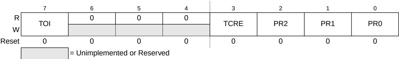
Figure 19-16. Timer System Control Register 2 (TSCR2)
