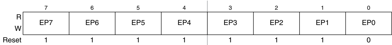
Figure 3-15. EEPROM Page Index Register (EPAGE)
