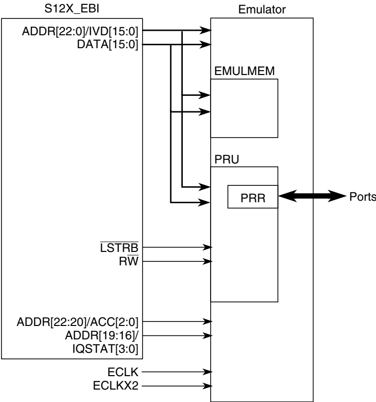
Figure 5-5. Application in Emulation Single-Chip Mode
