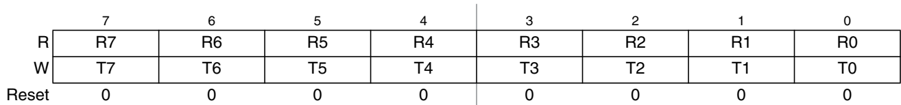
Figure 20-13. SCI Data Registers (SCIDRL)
