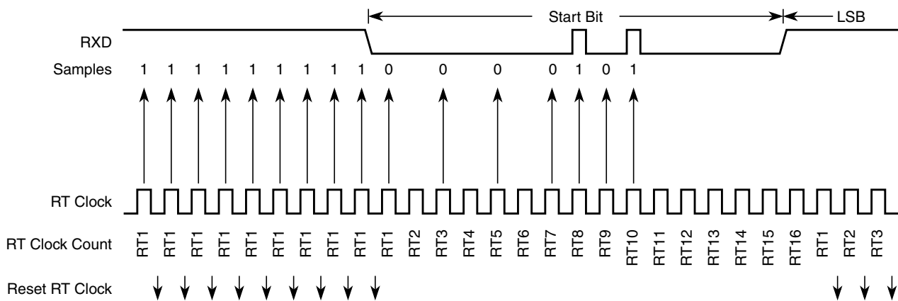
In Figure 20-27 , a noise burst makes the majority of data samples RT8, RT9, and RT10 high. This sets the noise flag but does not reset the RT clock. In start bits only, the RT8, RT9, and RT10 data samples are ignored.
