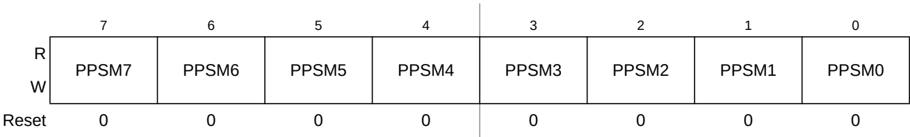
Figure 23-37. Port M Polarity Select Register (PPSM)
