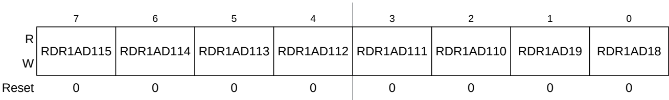
Figure 23-73. Port AD1 Reduced Drive Register 1 (RDR1AD1)
