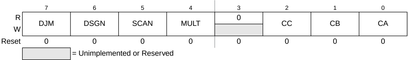
Figure 5-8. ATD Control Register 5 (ATDCTL5)
