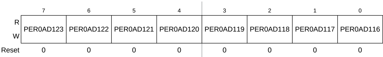
Figure 23-74. Port AD1 Pull Up Enable Register 0 (PER0AD1)
