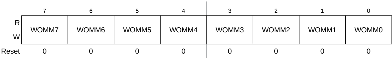
Figure 23-38. Port M Wired-OR Mode Register (WOMM)
