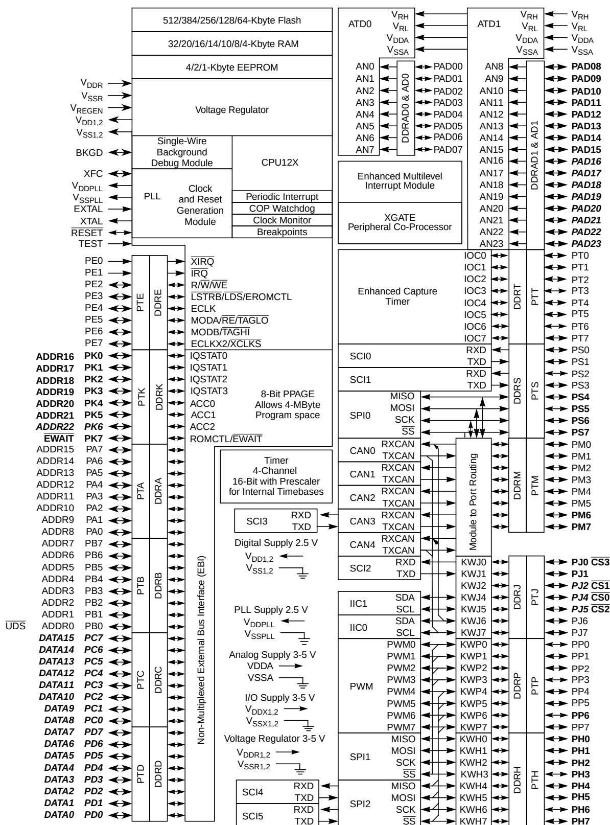
Figure 1-1. MC9S12XD-Family Block Diagram
