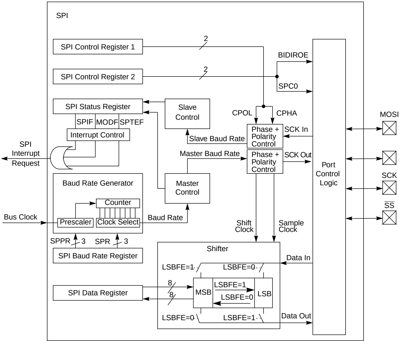
Figure 12-1. SPI Block Diagram
