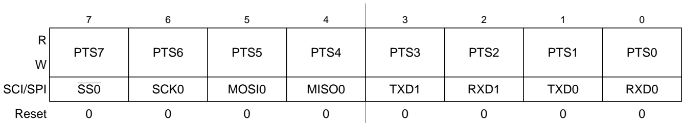
Figure 23-25. Port S Data Register (PTS)
