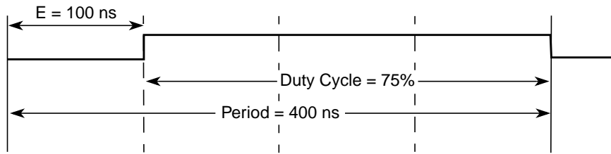
Figure 8-21. PWM Left Aligned Output Example Waveform
