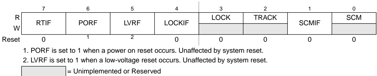
Figure 2-7. CRG Flags Register (CRGFLG)
