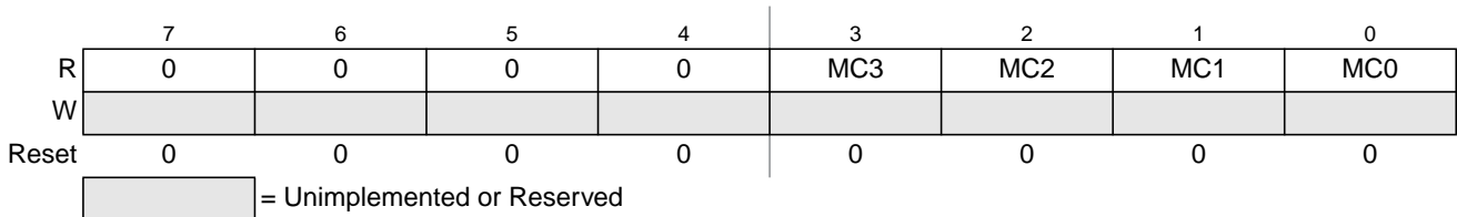
Figure 20-12. Debug Match Flag Register (DBGMFR)
