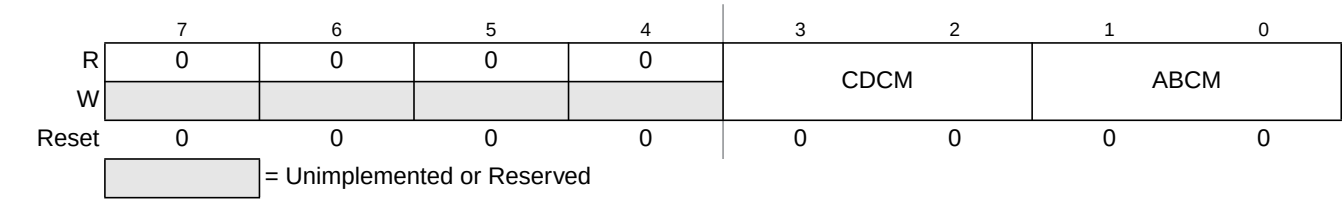
Figure 20-6. Debug Control Register2 (DBGCR2)
