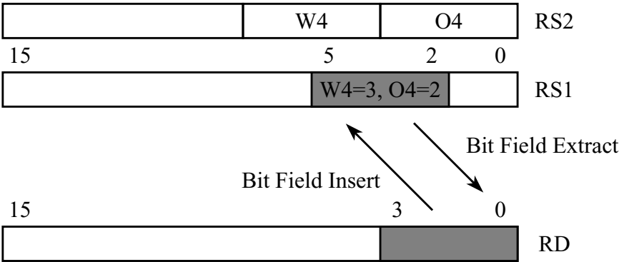
Figure 6-23. Bit Field Addressing
