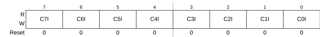
Figure 7-15. Timer Interrupt Enable Register (TIE)
