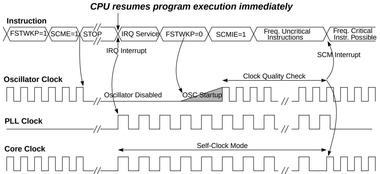
Figure 2-24. Fast Wake-up from Full Stop Mode: Example 2
