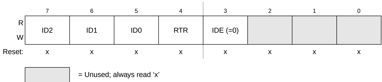
Figure 10-31. Identifier Register 1 — Standard Mapping
