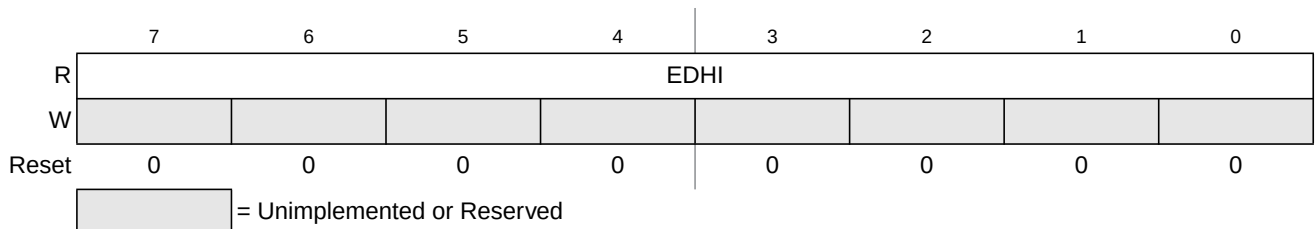
Figure 25-15. EEPROM Data High Register (EDATAHI)
