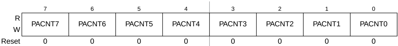
Figure 7-40. Pulse Accumulators Count Register 0 (PACN0)
