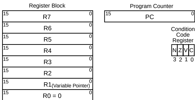
Figure 6-19. Programmer's Model
