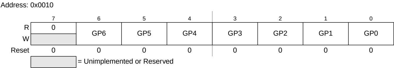
Figure 17-6. Global Page Index Register (GPAGE)
