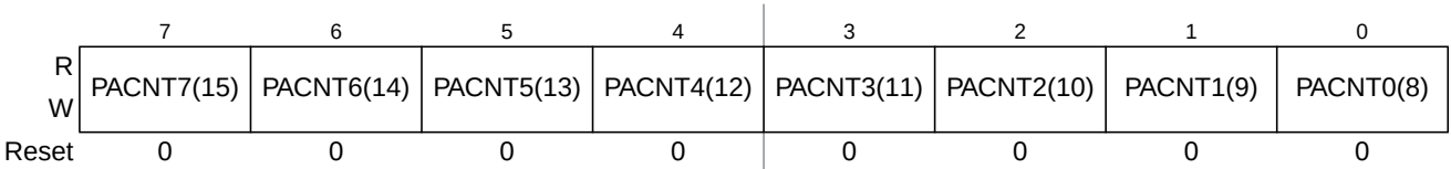
Figure 7-39. Pulse Accumulators Count Register 1 (PACN1)
