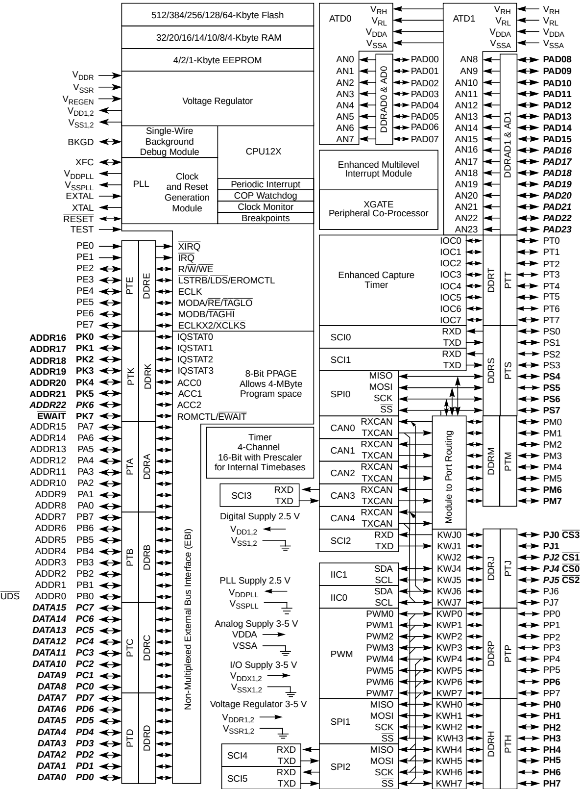
Figure 1-1. MC9S12XD-Family Block Diagram
