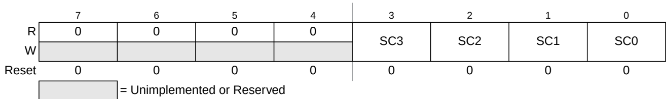
Figure 20-10. Debug State Control Register 2 (DBGSCR2)
