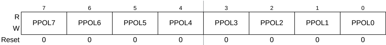
Figure 8-4. PWM Polarity Register (PWMPOL)
