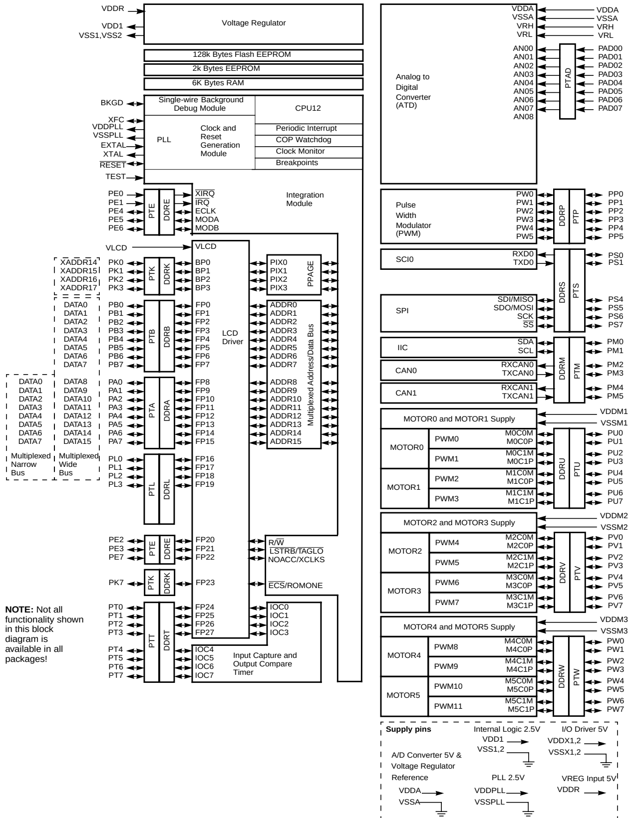
Figure 1-2 MC9S12H128 Block Diagram
