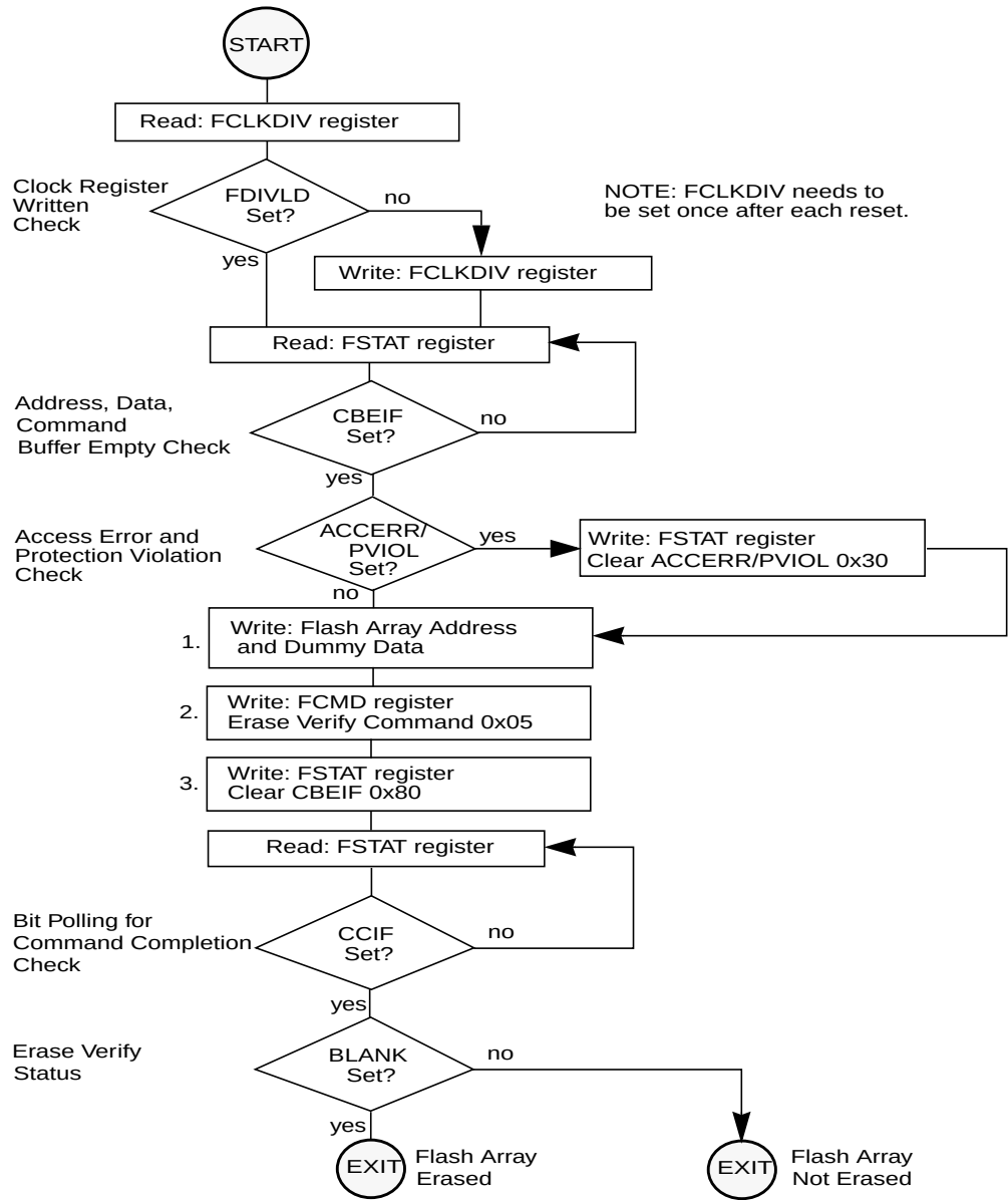
Figure 2-22. Example Erase Verify Command Flow
