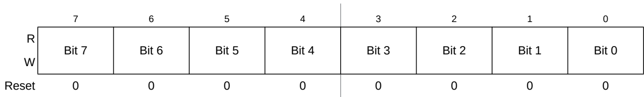
Figure 16-18. Debug Comparator A Register Low (DBGCAL)
