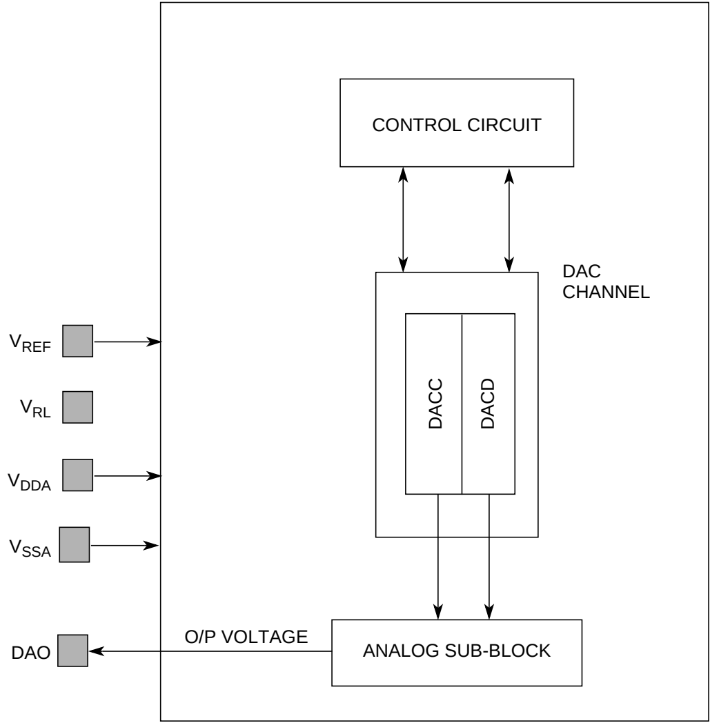
Figure 7-1. DAC8B1C Functional Block Diagram
