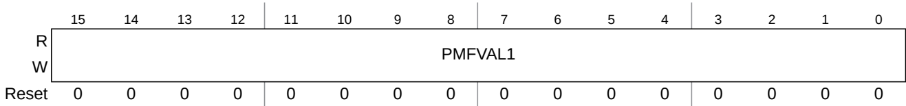
Figure 11-21. PMF Value 1 Register (PMFVAL1)
