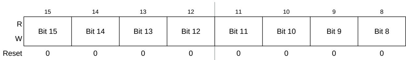
Figure 16-17. Debug Comparator A Register High (DBGCAH)
