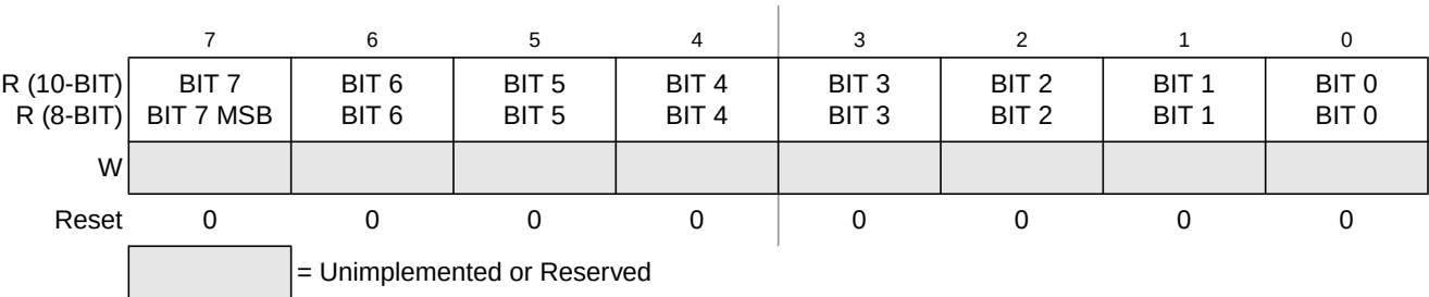
Figure 6-21. Right Justified, ATD Conversion Result Register x, Low Byte (ATDDRxL)
