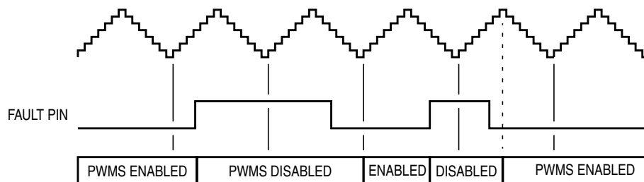
Figure 11-76. Automatic Fault Clearing
