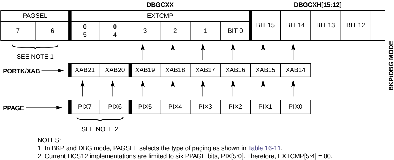
Figure 16-10. Comparator C Extended Comparison in BKP/DBG Mode
