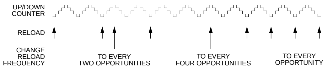
Figure 11-65. Full Cycle Reload Frequency Change
