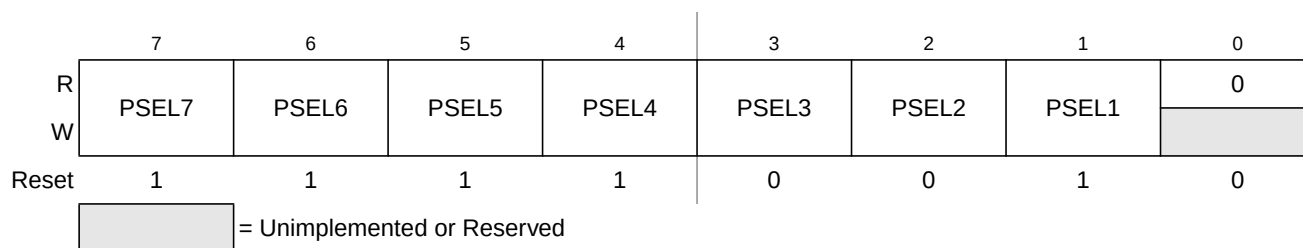
Figure 17-4. Highest Priority I Interrupt Register (HPRIO)
