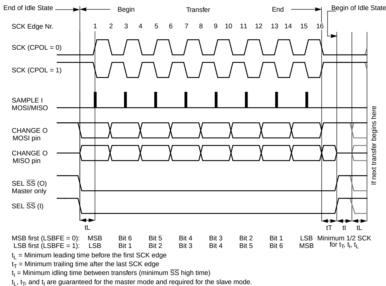
Figure 9-9. SPI Clock Format 0 (CPHA = 0)
