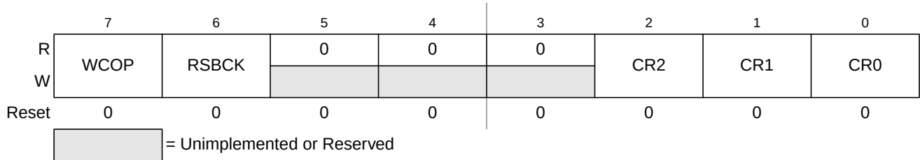
Figure 4-12. CRG COP Control Register (COPCTL)
