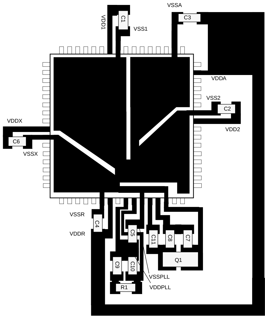
Figure 1-13. Recommended PCB Layout (64-QFN)
