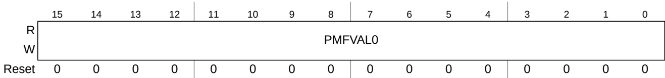
Figure 11-20. PMF Value 0 Register (PMFVAL0)
