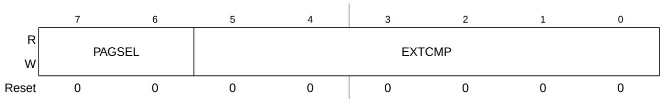
Figure 16-9. Debug Comparator C Extended Register (DBGCCX)
