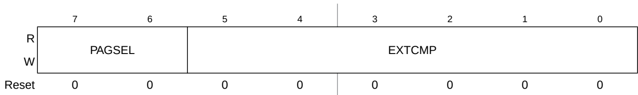
Figure 16-19. Debug Comparator B Extended Register (DBGCBX)
