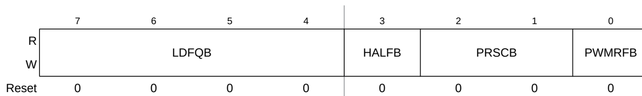
Figure 11-32. PMF Frequency Control B Register (PMFFQCB)
