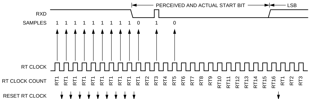
Figure 8-19. Start Bit Search Example 4
