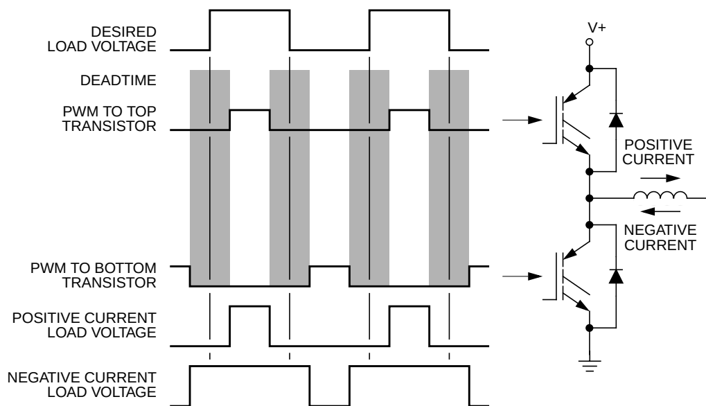
Figure 11-53. Deadtime Distortion
