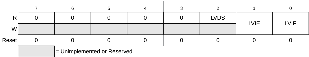
Figure 14-2. VREG3V3 — Control Register (VREGCTRL)
