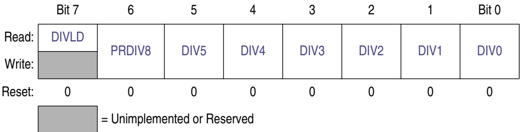
Figure 4-4. FLASH Clock Divider Register (FCDIV)
