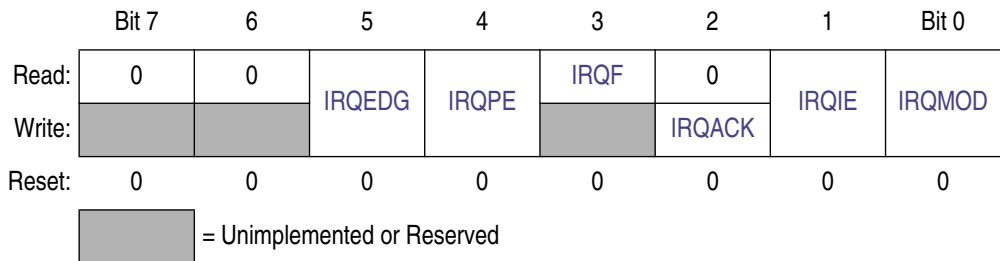
Figure 5-2. Interrupt Request Status and Control Register (IRQSC)
