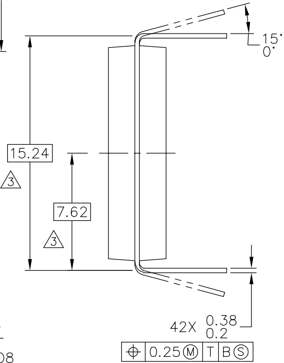
END VIEW
