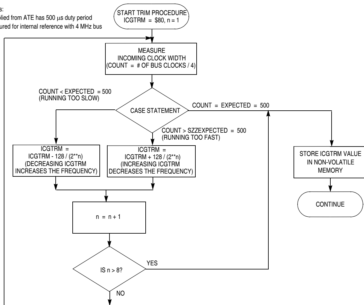
Figure 7-11. Trim Procedure
