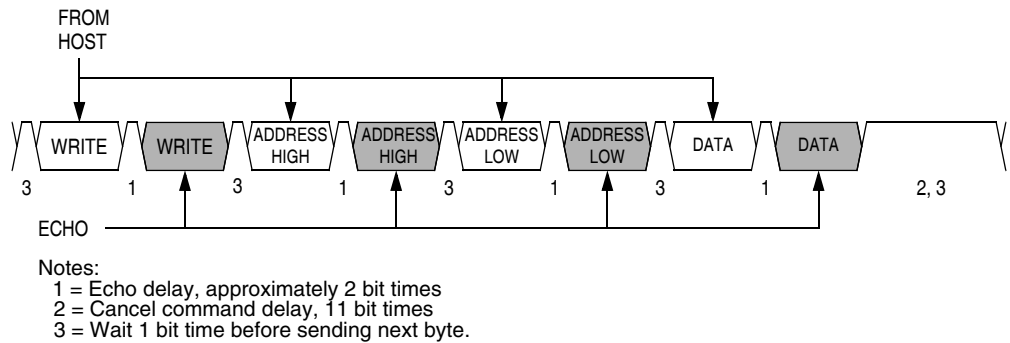
Figure 17-16. Write Transaction
