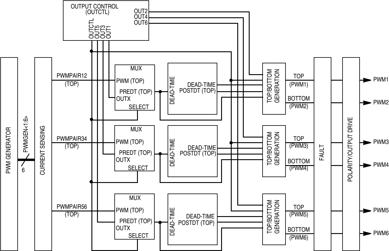
Figure 12-14. Dead-Time Generators
