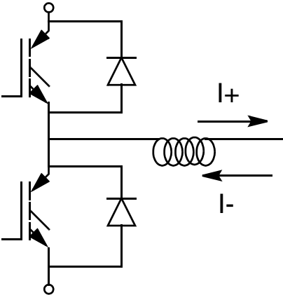
Figure 12-19. Current Convention
