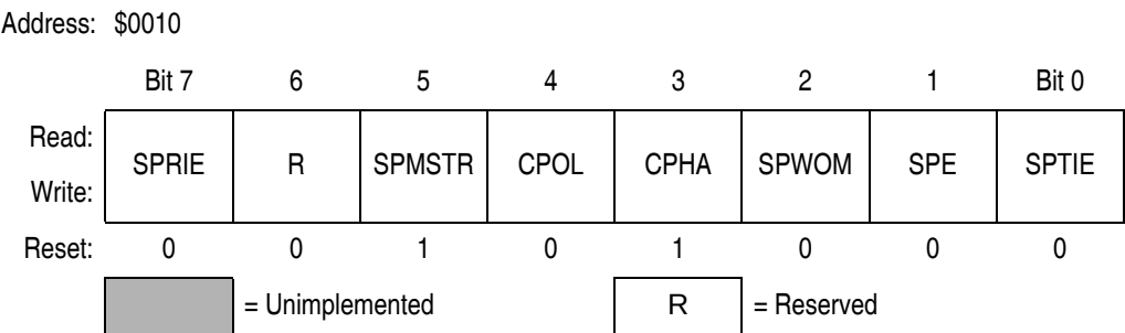
Figure 14-13. SPI Control Register (SPCR)
