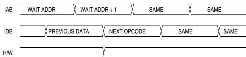
Figure 4-15. Wait Mode Entry Timing
