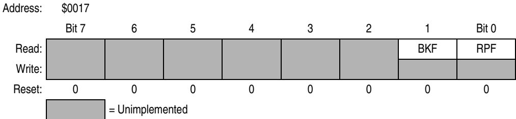
Figure 7-14. SCI Status Register 2 (SCS2)
