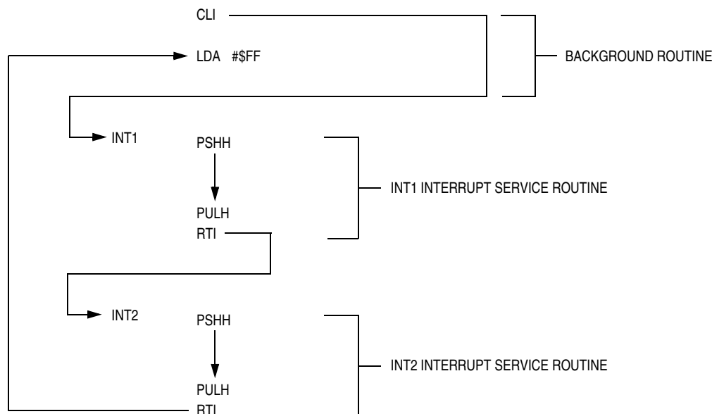
Figure 4-11. Interrupt Recognition Example
