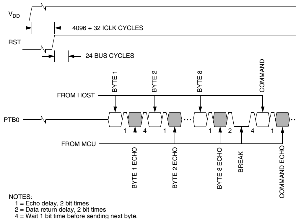
Figure 16-14. Monitor Mode Entry Timing
