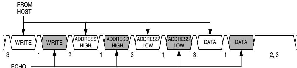
Figure 18-14. Read Transaction
