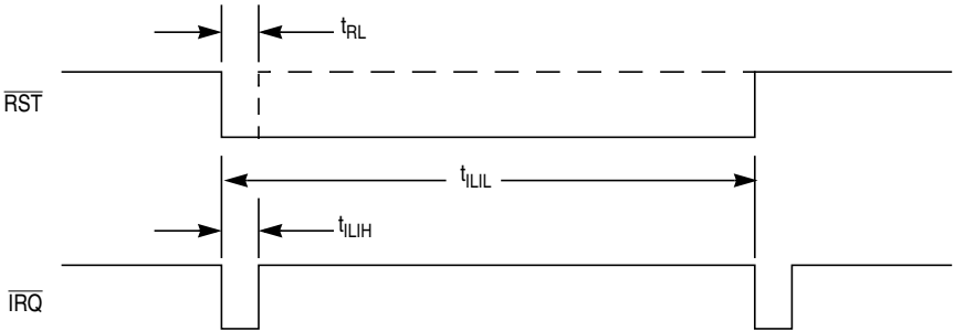
Figure 19-1. \overline{RST} and \overline{IRQ} Timing
