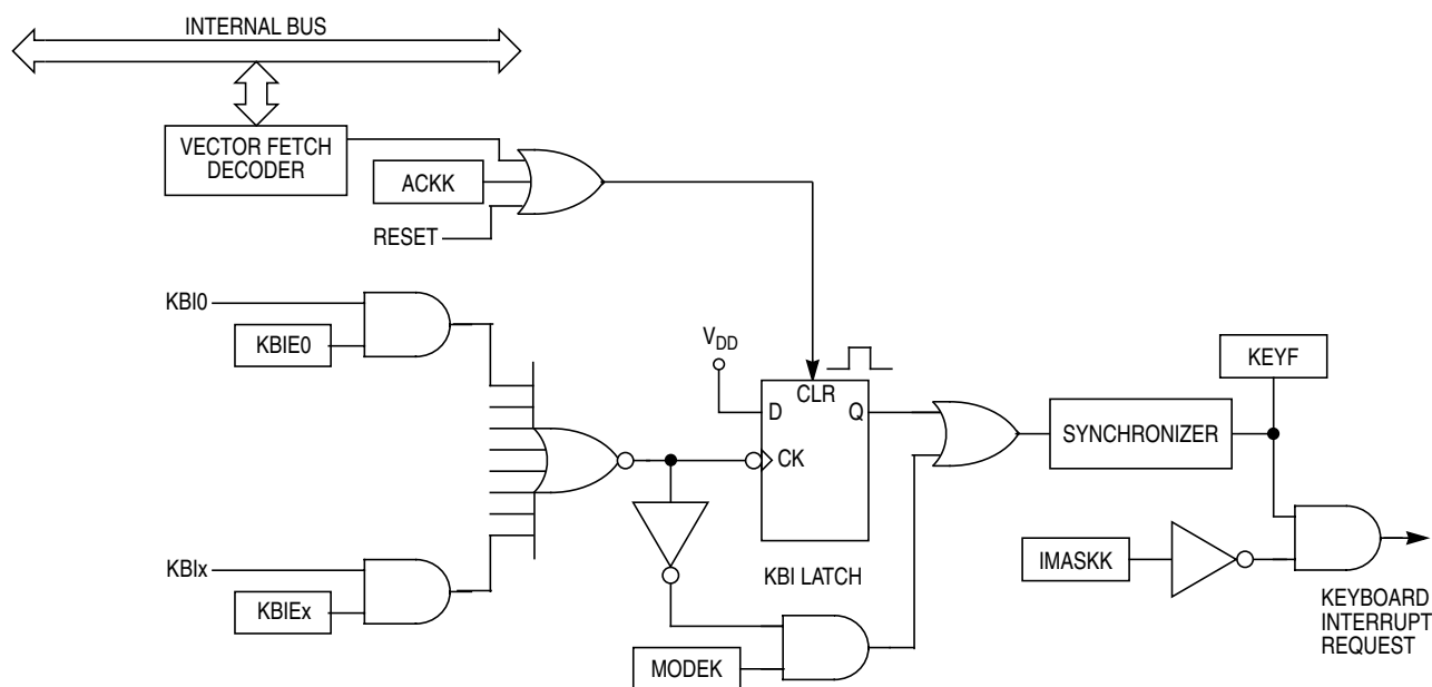
Figure 10-1. Keyboard Interrupt Block Diagram
