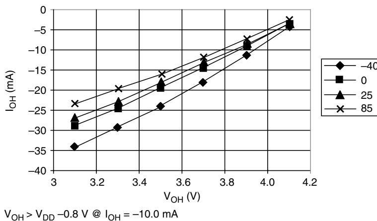
Figure 19-4. Typical High-Side Driver Characteristics – Port PTC4–PTC0 ( V_{DD} = 4.5 \text{ Vdc} )
