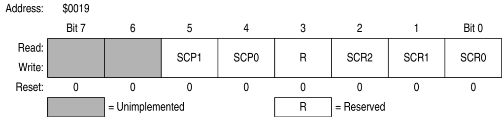
Figure 13-16. SCI Baud Rate Register (SCBR)
