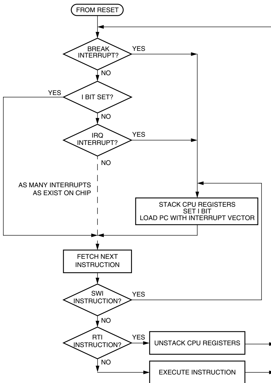
Figure 14-10. Interrupt Processing
