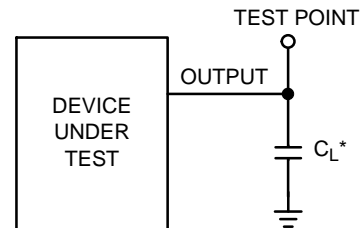
Figure 3. Test Circuit
