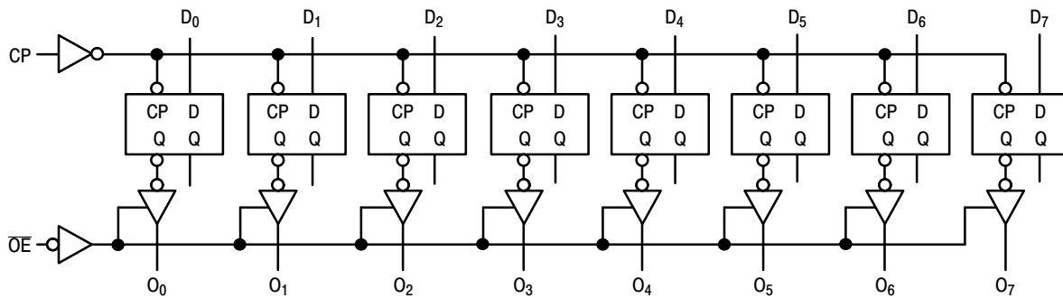
Figure 3. Logic Diagram
