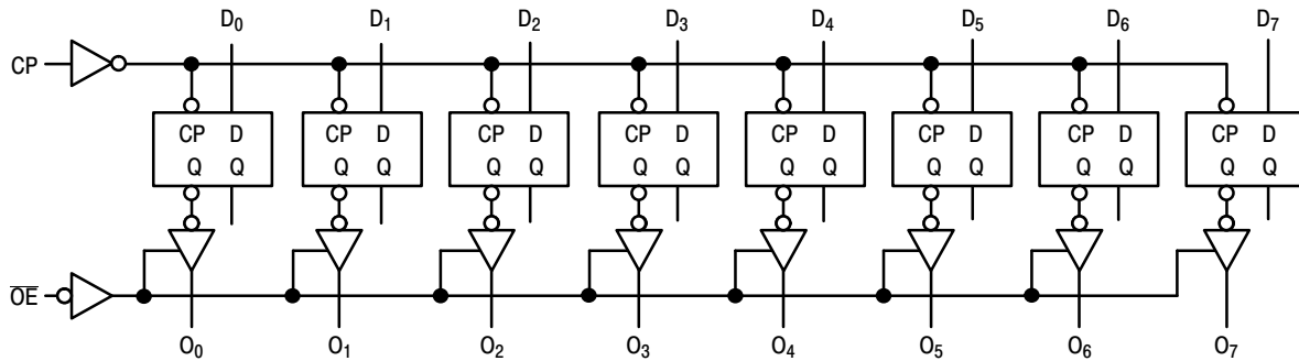
Figure 3. Logic Diagram
