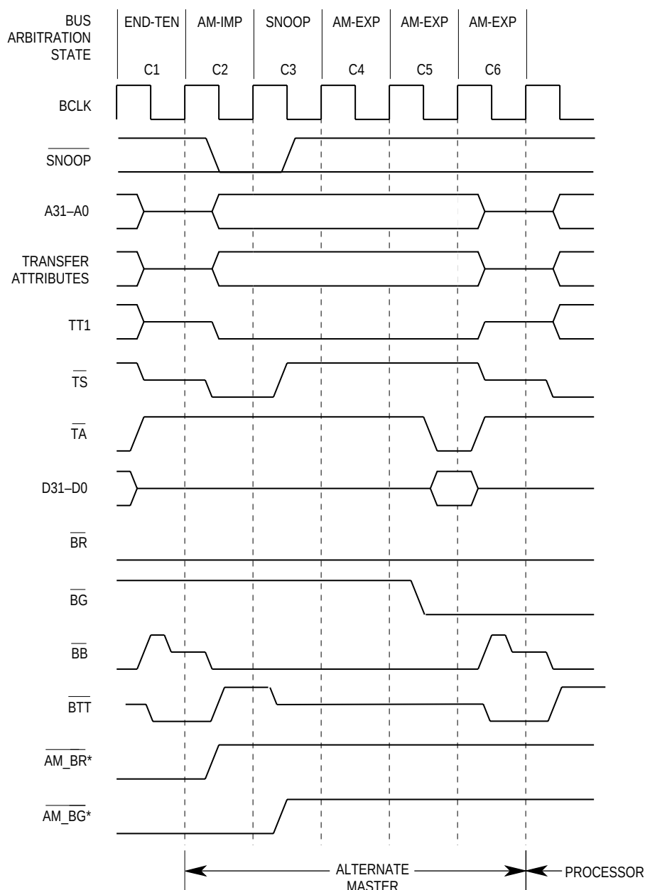
Figure 7-47. Snooped Bus Cycle
