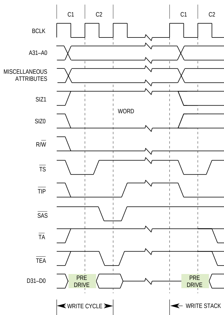
Figure 7-37. Word Write Access Bus Cycle Terminated with \overline{\text{TEA}} Timing
