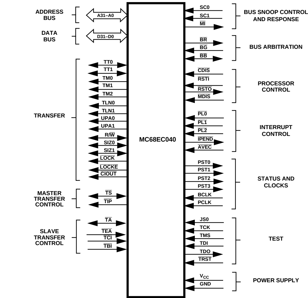
Figure B-3. MC68EC040 Functional Signal Groups
