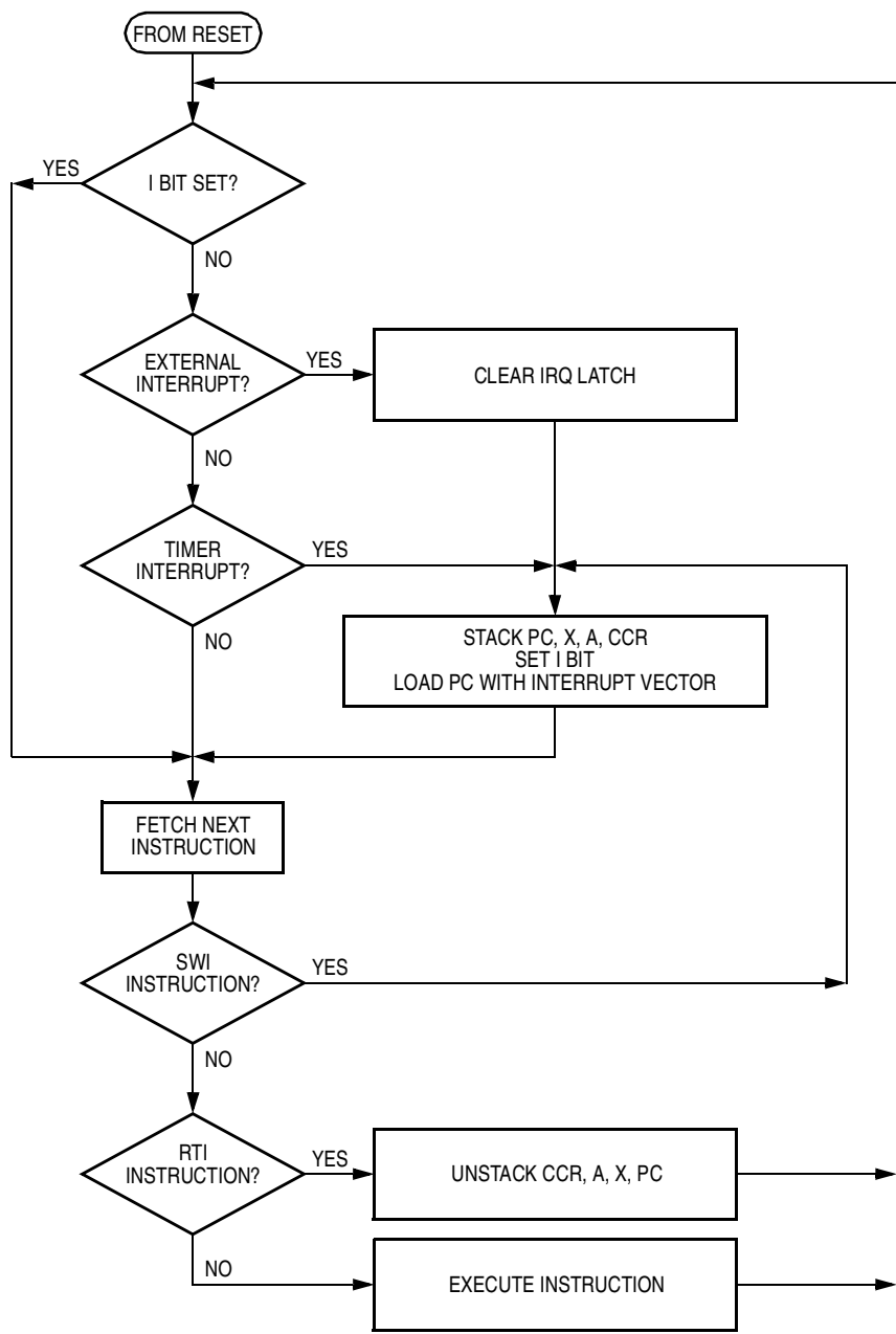
Figure 4-7. Interrupt Flowchart
