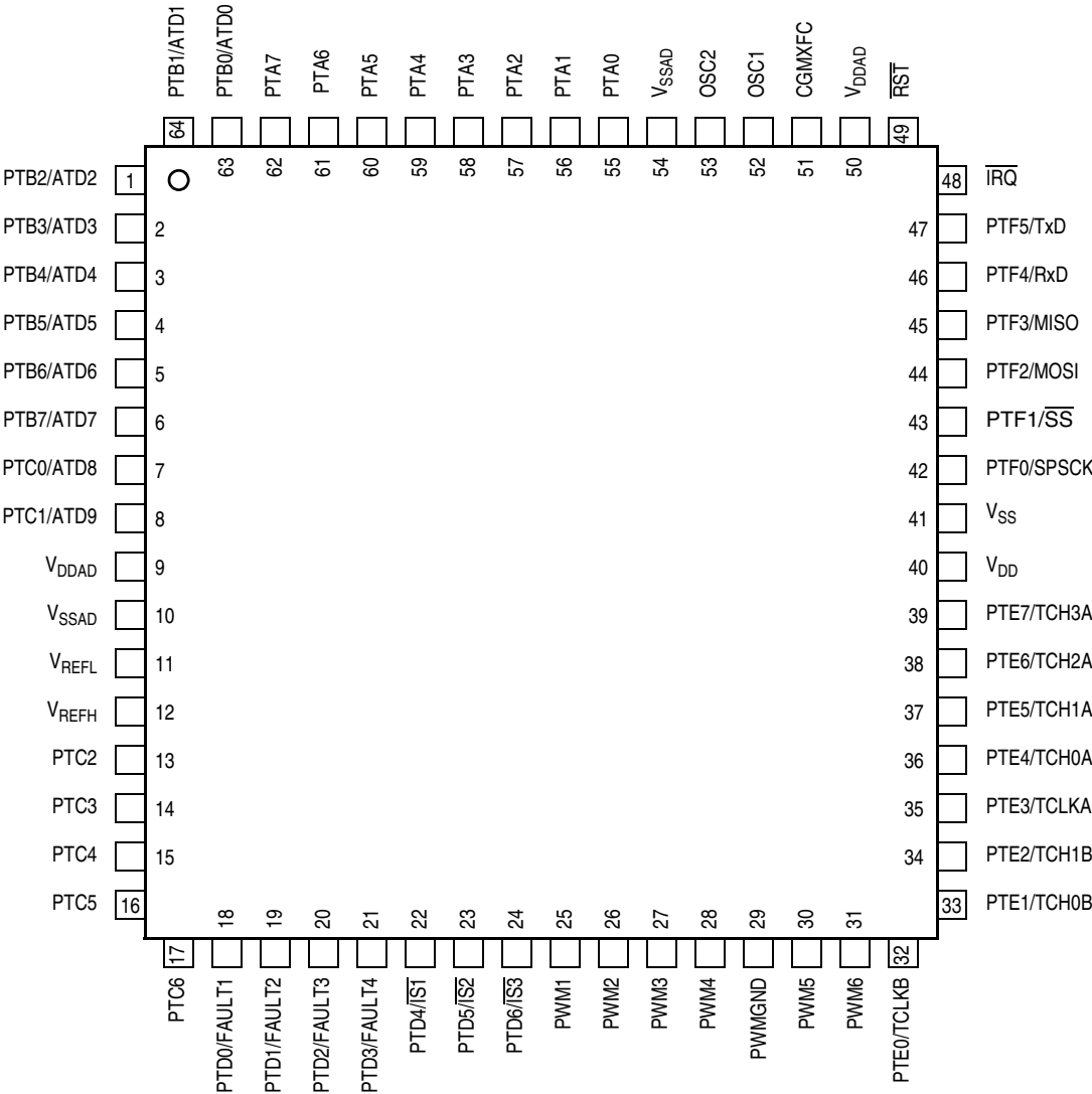
Figure 1-2. 64-Pin QFP Pin Assignments
