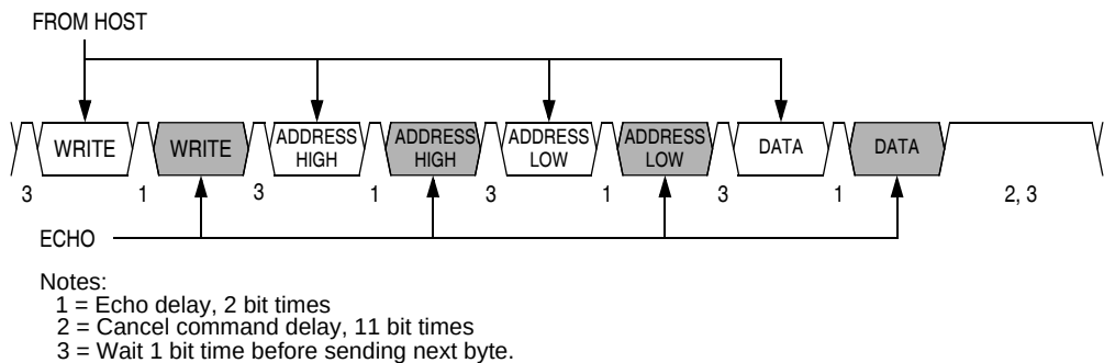
Figure 10-6. Write Transaction
