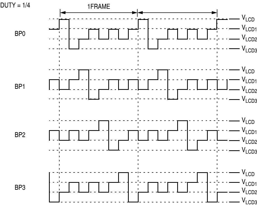
Figure 16-7. 1/4 Duty LCD Backplane Driver Waveforms
