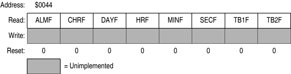
Figure 12-5. RTC Status Register (RTCSR)
