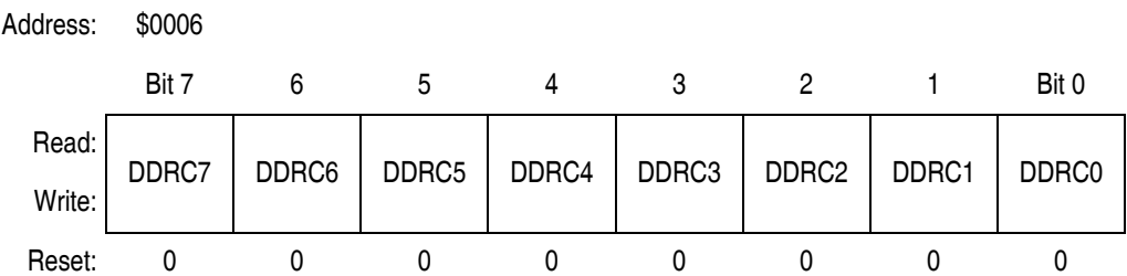
Figure 17-10. Data Direction Register B (DDRB)
