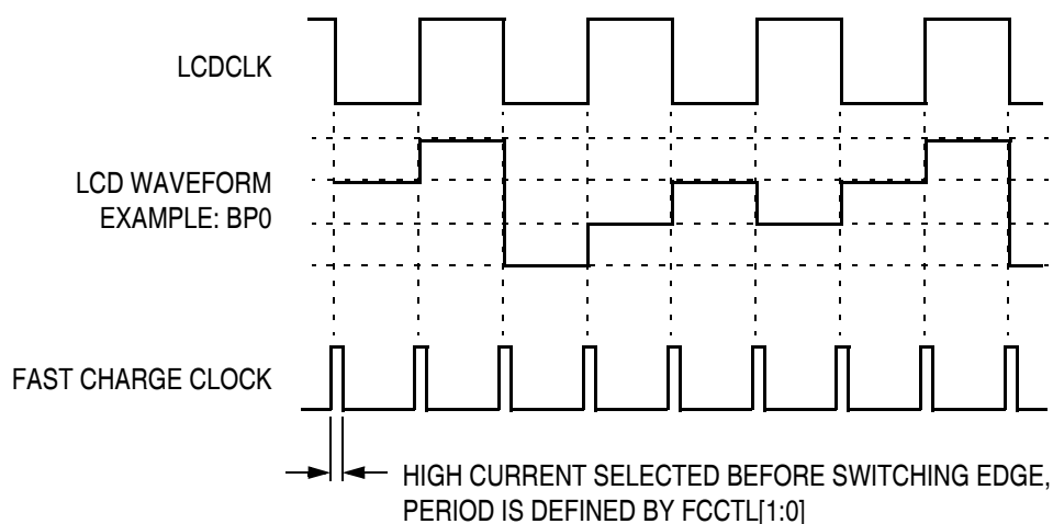
Figure 16-4. Fast Charge Timing
