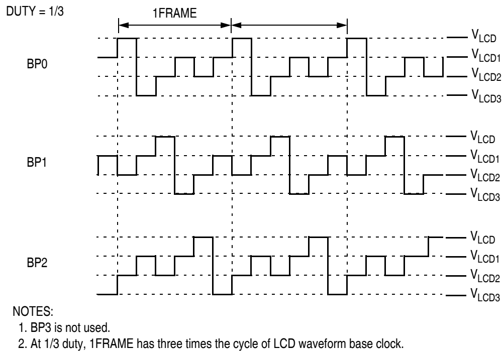
Figure 16-5. 1/3 Duty LCD Backplane Driver Waveforms
