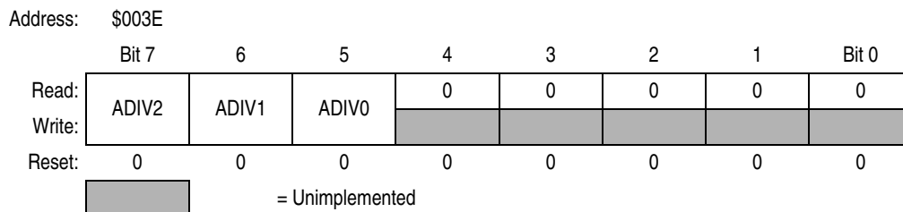
Figure 10-5. ADC Input Clock Register (ADICK)
