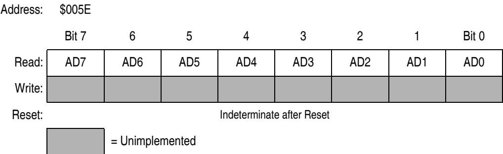
Figure 12-3. ADC Data Register (ADR)
