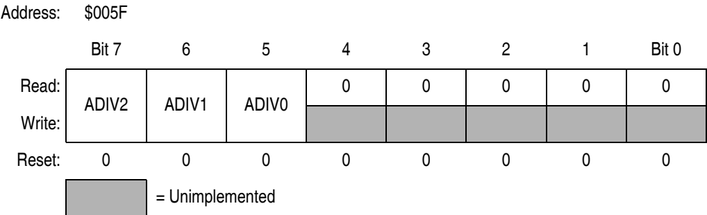
Figure 12-4. ADC Input Clock Register (ADICLK)
