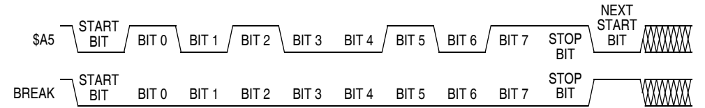
Figure 9-3. Sample Monitor Waveforms
