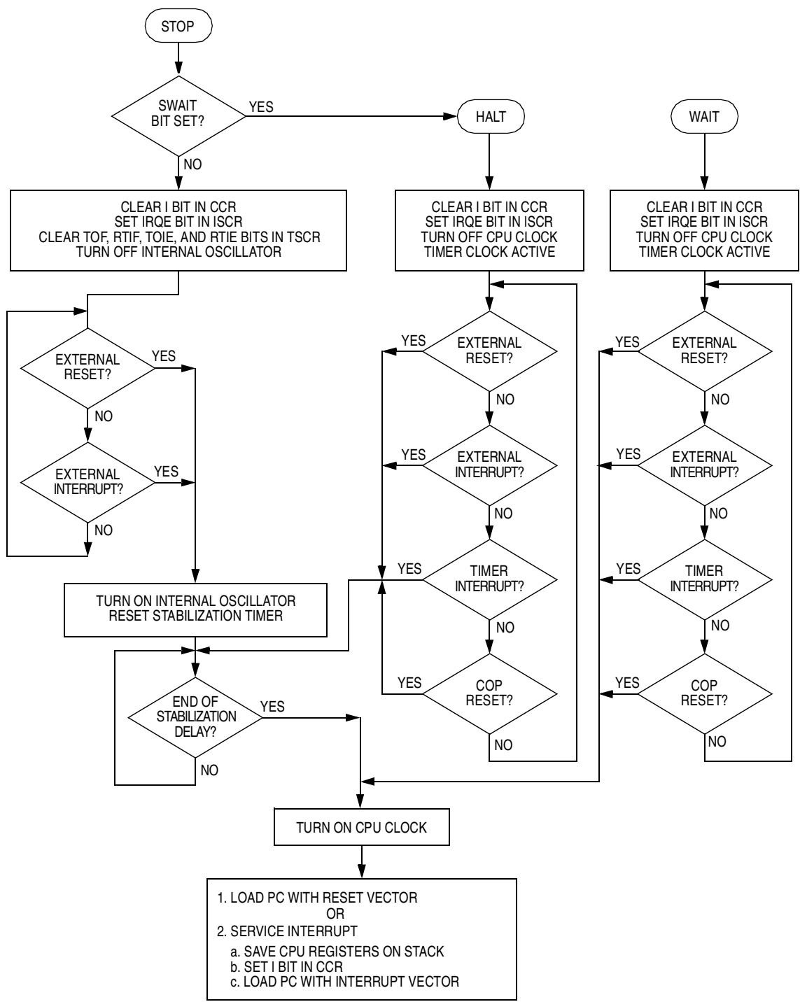
Figure 5-2. Stop/Halt/Wait Flowchart
